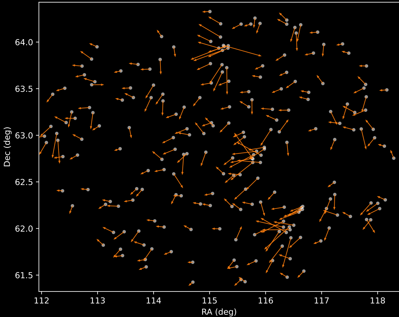
APOGEE DR17 Cluster 2 Proper Motion Vectors (n=216)
