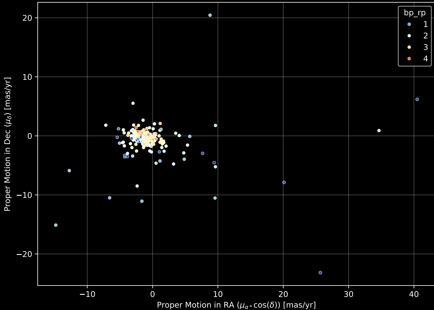
APOGEE DR17 Field: [124+00] Proper Motion Diagram (n= 282)
