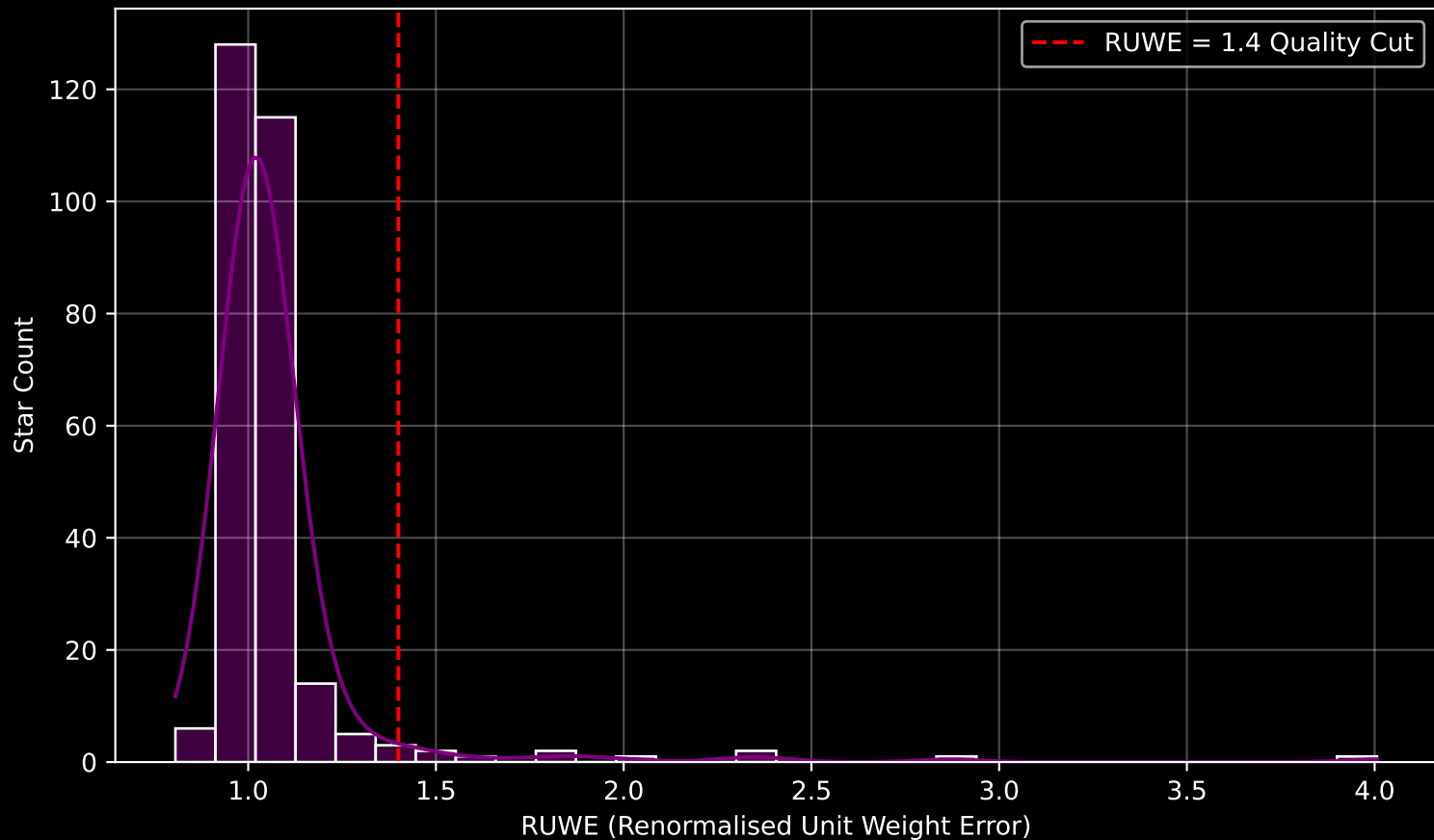
GAPOGEE DR17 Field [124+00] RUWE Distribution (n= 281)
