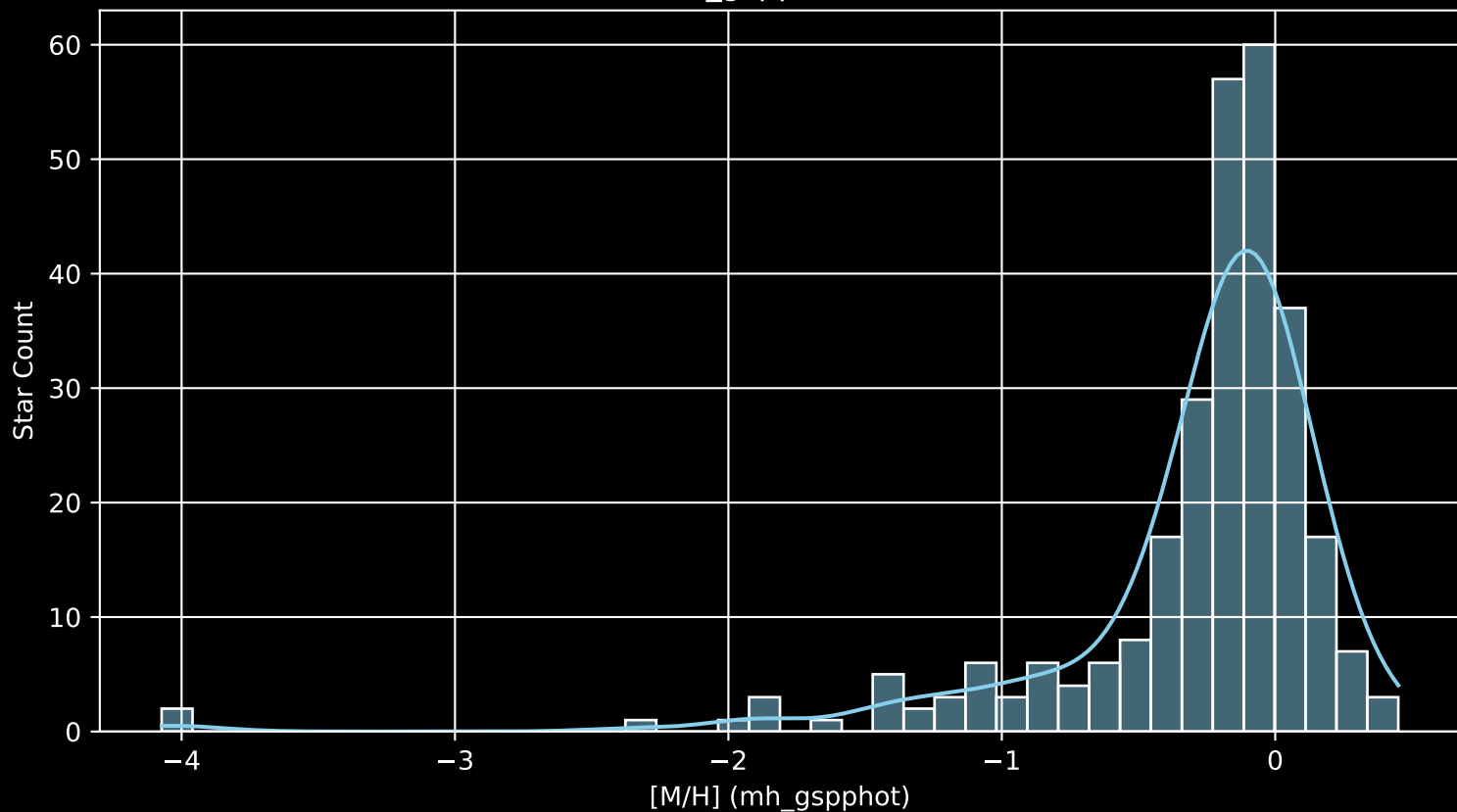
APOGEE DR17 Field: [124+00 [M/H] (mh_gspphot) (n= 278)
