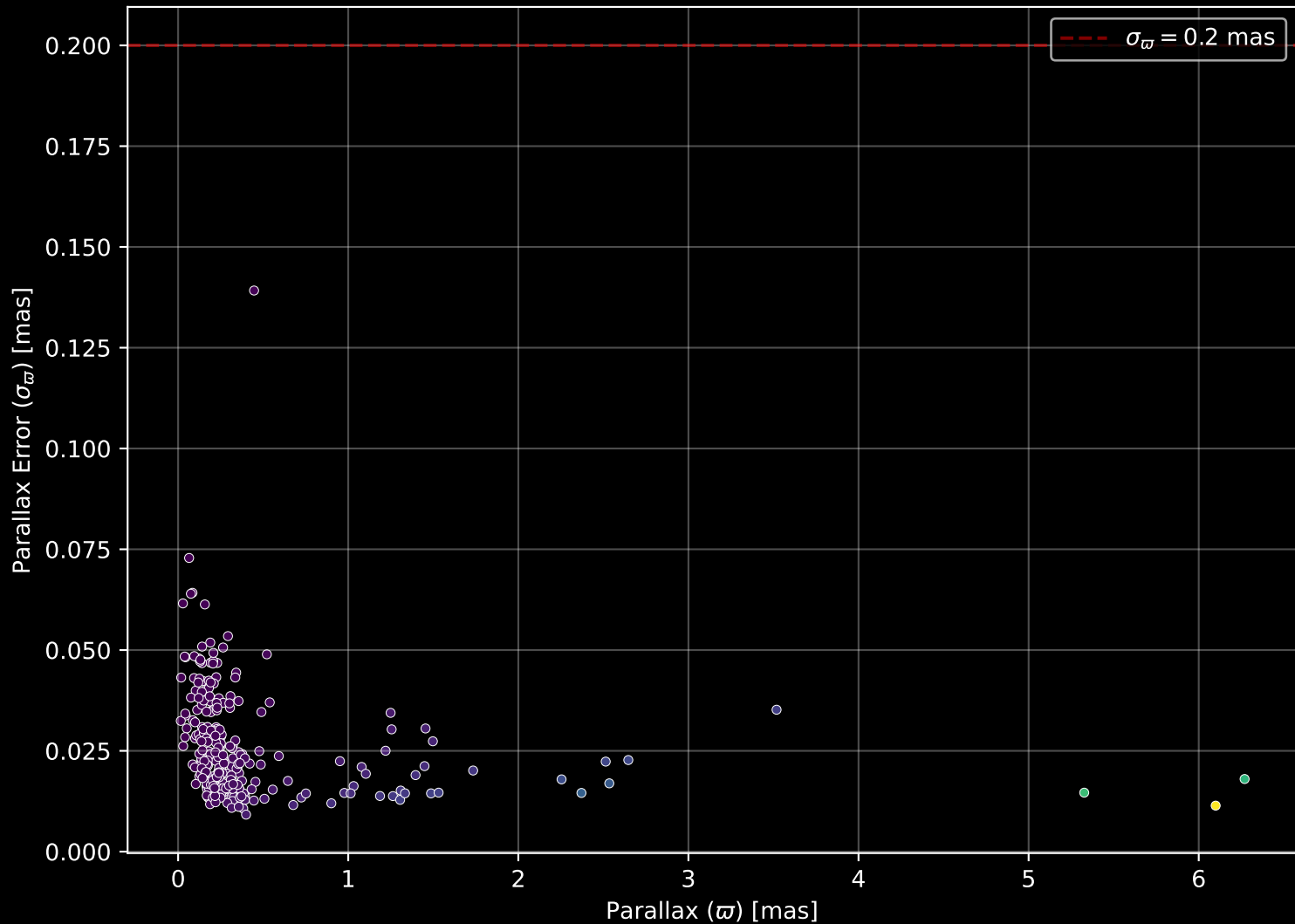
APOGEE DR17 Field: [124+00] Parallax Quality (n= 282)
