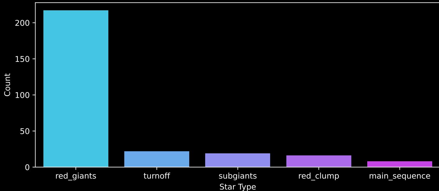
APOGEE DR17 Field: [124+00] Count plot of Star Type
